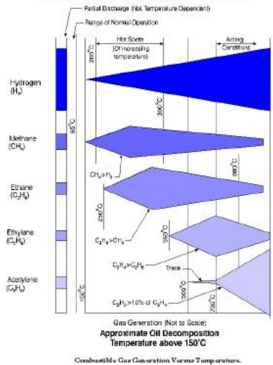
Combustible Gas Generation vs. Approximate Oil Decomposition Temperature
