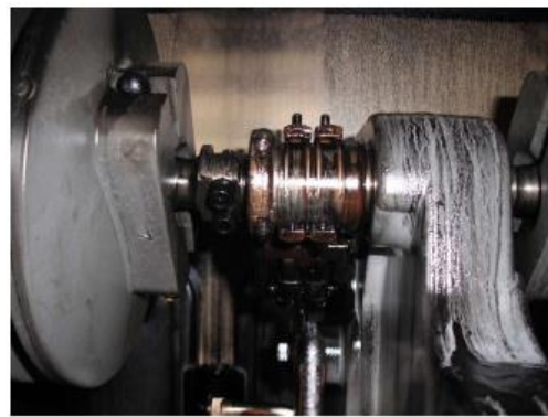
Film on Reversing Switch Contact
